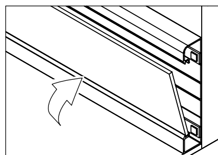
6 Press the diffuser against the back plate until it clicks into place.
