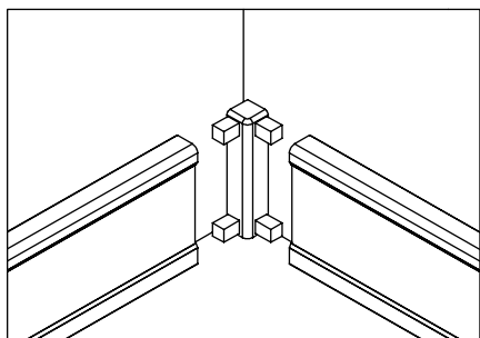
7 Apply adhesive to the internal corners to secure them in position.
