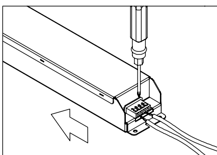
5 Connect the LED strips and the driver and the driver to the mains. Cables can be carried within the profiles for multi-drive connections. Consult local electricians to obtain accurate results.
