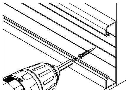
3 Screw the wall fixation parts to the places that are drilled at 50cm intervals.
