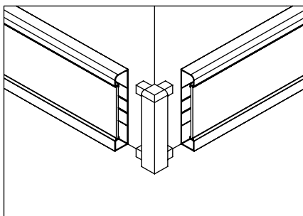
8 Apply adhesive to the external corners to secure them in position.
