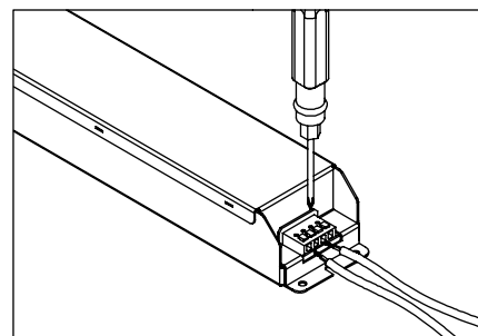
6 Connect the LED strips and the driver and the driver to the mains. Cables can be carried within the profiles for multi-drive connections. Consult local electricians to obtain accurate results.
